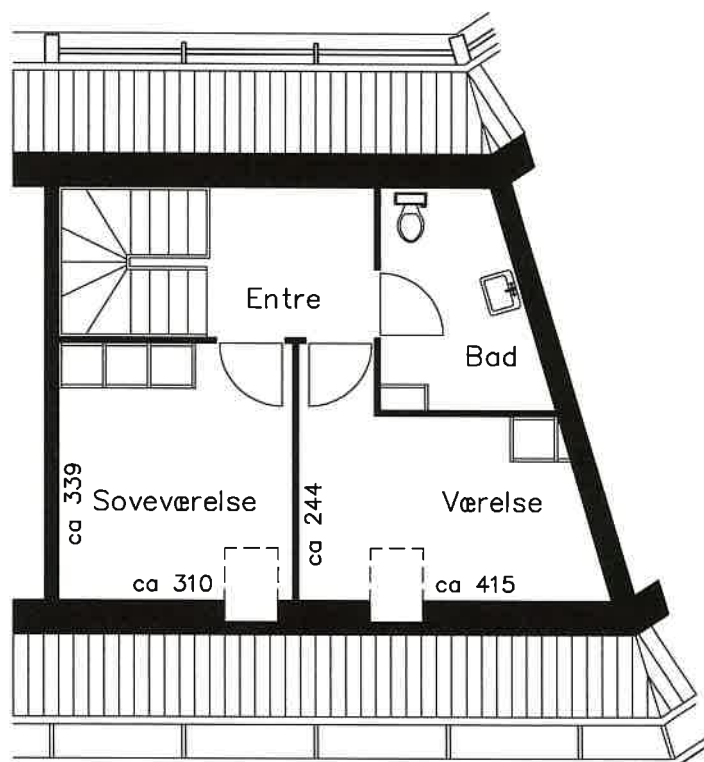
4. sals plan
